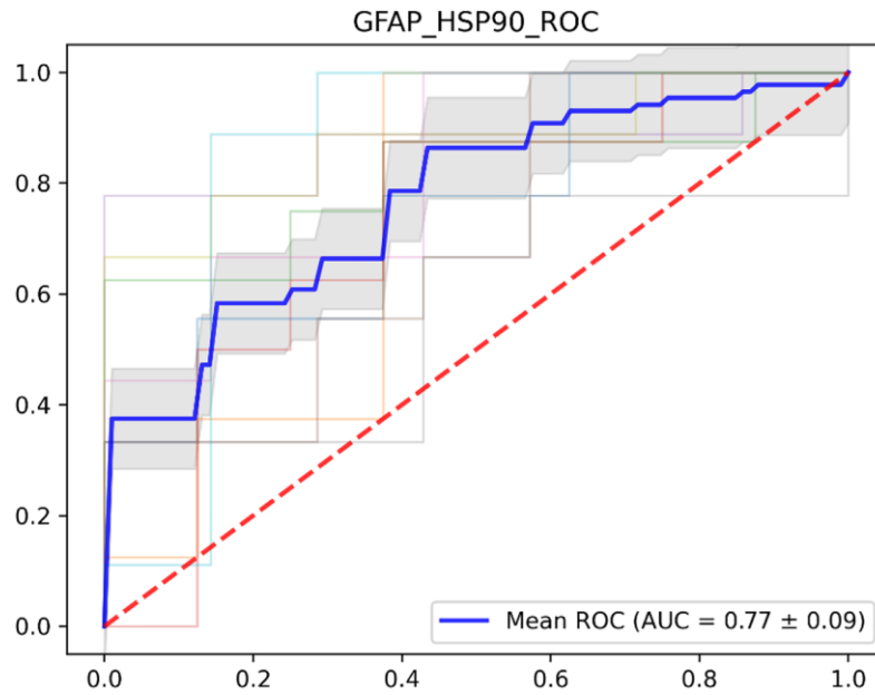
Supplementary Figure 2. Results of ten-fold cross validation of support vector machine model in GFAP and HSP90AB1 combination.
