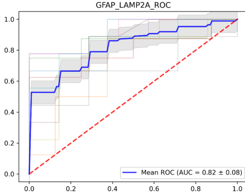
Supplementary Figure 1. Results of ten-fold cross validation of support vector machine model in GFAP and LAMP2A combination.
