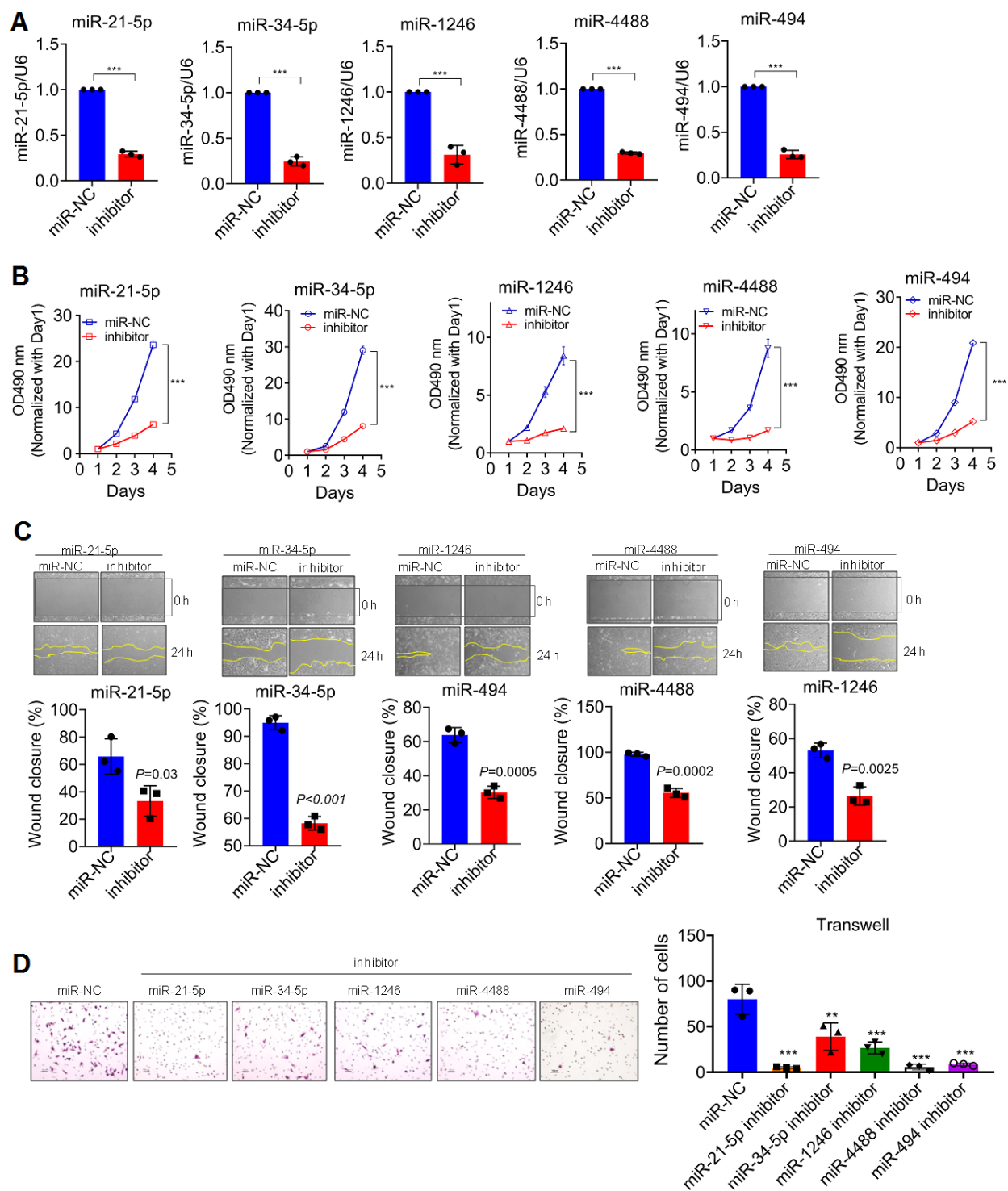
Figure 5. DGCR8 produces a pro-growth miRNA Profile that promotes Cell Proliferation. (A) knock-down efficiency detected by qRT-PCR of transient silencing of miRNA that down-regulated in T87G cells when DGCR8 was knocked down. miR-NC, miR-scramble; Inhibitor, a contraction of miRNA inhibitor. Two-tailed, unpaired T-test was used to analyze the significant difference (miR-21-5p, t=38.44 , df=4 , P<0.0001 ; miR-34-5p, t=26.19 , df=4 , P<0.0001 ; miR-1246, t=11.66 , df=4 , P<0.0001 ; miR-4488, t=16.9 , df=4 , P<0.0001 ; miR-494, t=28.33 , df=4 , P<0.0001 ). Here *** P<0.0001 compared with control. (B) MTT assay was performed on T87G cells whose endogenous miRNAs, as shown, were transiently knocked down. Two-tailed, unpaired T-test was used to analyze the significant difference, *** P<0.001 compared with control. (C) Wound closure assay was conducted in parallel with MTT assays to appraise the migratory variation in T87G cells. Two-tailed, independent T-test was used to analyze the significant difference. (D) Transwell assays were carried out to analyze the invasive variation after differential miRNAs were transiently knocked down in T87G cells. One way ANOVA (Bonferroni approach) was taken to analyze the significant difference among groups in comparison with control group transfected with miR-NC. Here, ** P<0.001 , *** P<0.0001 relative to control.
