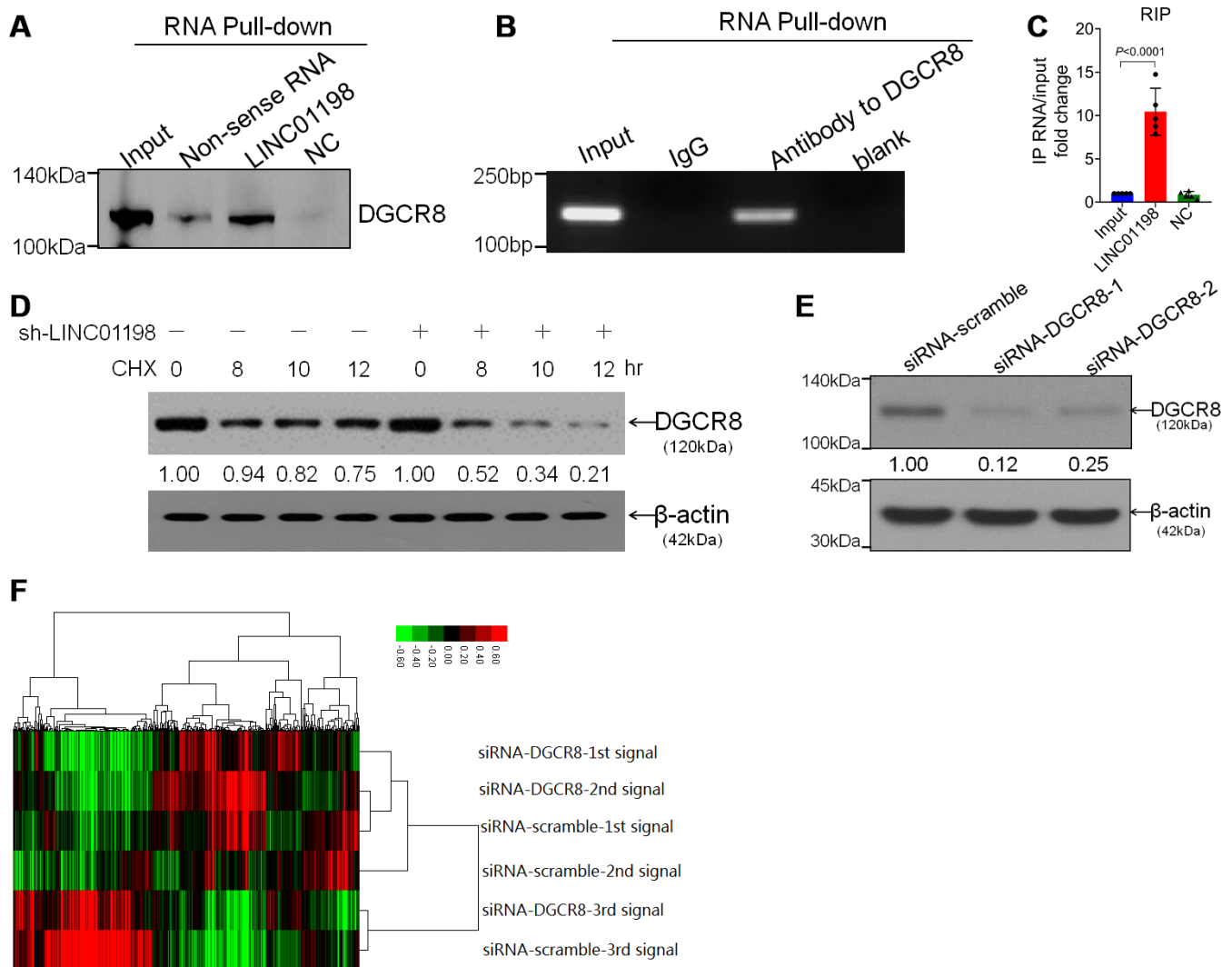
Figure 4. LINC01198 interacted with DGCR8 stabilizing DGCR8. (A) Immunoblotting detection of DGCR8 in the LINC01198 pull-down complex. LINC01198 fragment (hereafter referred to as LINC01198) was labeled with the biotin; Non-sense RNA was labeled with the biotin whose length was similar to that of LINC01198 fragment; NC was the LINC01198 without biotin label. The molecular weight of DGCR8 approximates 120 kilodalton (kDa), suggested by manufacturer's instruction that accompanies. (B) The PCR product of RNA immunoprecipitation (RIP), run by agarose gel electrophoresis with 12% separating gel. (C) qRT-PCR verified that LINC01198 was accumulated in DGCR8-precipitated protein sample. Two-tailed, independent sample T-test was used to analyze the significant difference ( t=7.794 , df=8 , P<0.0001 ). (D) immunoblotting detection of DGCR8 stability in the presence of Cycloheximide (CHX) at 12.5\mu\text{g/mL} in T87G cells transfected with or without sh-LINC01198. gray density was quantitated by Image J (NIH, Bethesda, MA, USA). (E) Knock down efficiency of siRNA to DGCR8 at two different interfering sites, as evaluated by western-blot. Shown were the representative ones singled out from candidates out of three independent experiments. (F) Cluster analysis of heat map of miRNA microarray (SurePrint, homo, Angilent, USA) performed on T87G and Hs 684 glioma cells transfected with siRNA to DGCR8. Transfection with siRNA-scramble was set as control.
