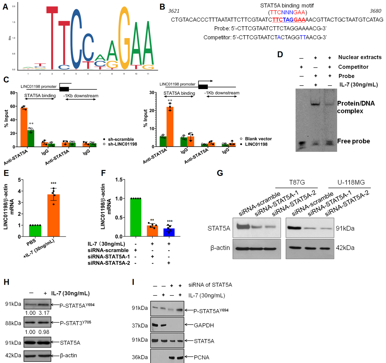
Figure 3. STAT5A identified as transcription factor that regulates the transcription of LINC01198. (A) Binding motif of STAT5A (TTCNNGAA, here N denotes any nucleotide) in the promoter of LINC01198, predicted by JASPAR ( http://jaspar.genereg.net/ ). (B) Representative binding position of STAT5A in the promoter of LINC01198 and the specific sequence of probe and its competitor probe involved in EMSA. (C) CHIP-qPCR analysis of transcriptional regulation of STAT5A on the promoter of LINC01198. Anti-STAT5A, CHIP-grade primary antibody to STAT5A; IgG, the isotype control of the primary antibody to STAT5A. The experiment was performed independently three times with triplicate in each time. Shown was the representative result. Two-tailed, independent sample T-test was used to analyze the significant difference. ** P < 0.01 compared with control. (D) EMSA analysis of the binding ability of STAT5A with the promoter of LINC01198. Here, competitor was the contraction of competitor probe. (E) Indirect regulation of STAT5A exerted by IL-7 (30ng/mL) over the expression of LINC01198 on mRNA level, as detected by qRT-PCR. (F) Similarly, indirect regulation of STAT5A exerted by IL-7 over the expression of LINC01198 on mRNA level in the presence of siRNA to STAT5A, as detected by qRT-PCR. Two-tailed, independent sample T-test was used to analyze the significant difference. ** P < 0.01 , *** P < 0.001 in comparison with control group. (G) immunoblotting detection of the knock-down efficiency of siRNA to STAT5A in T87G and U-118MG glioma cells, shown were the representative figures picked out of candidates we collected. (H) STAT5A can be specifically and appreciably activated at its 694 Tyrosine in the presence of IL-7 whereas STAT3 can hardly be phosphorylated. (I) activated STAT5A was capable of translocation from cytoplasm to nucleus in the presence of IL-7, as exemplified by western-blot. Of note, PCNA used as internal loading control for nuclear protein. All the experiments related to western-blot were performed independently three times and presented were the representative ones singled out from candidates.
